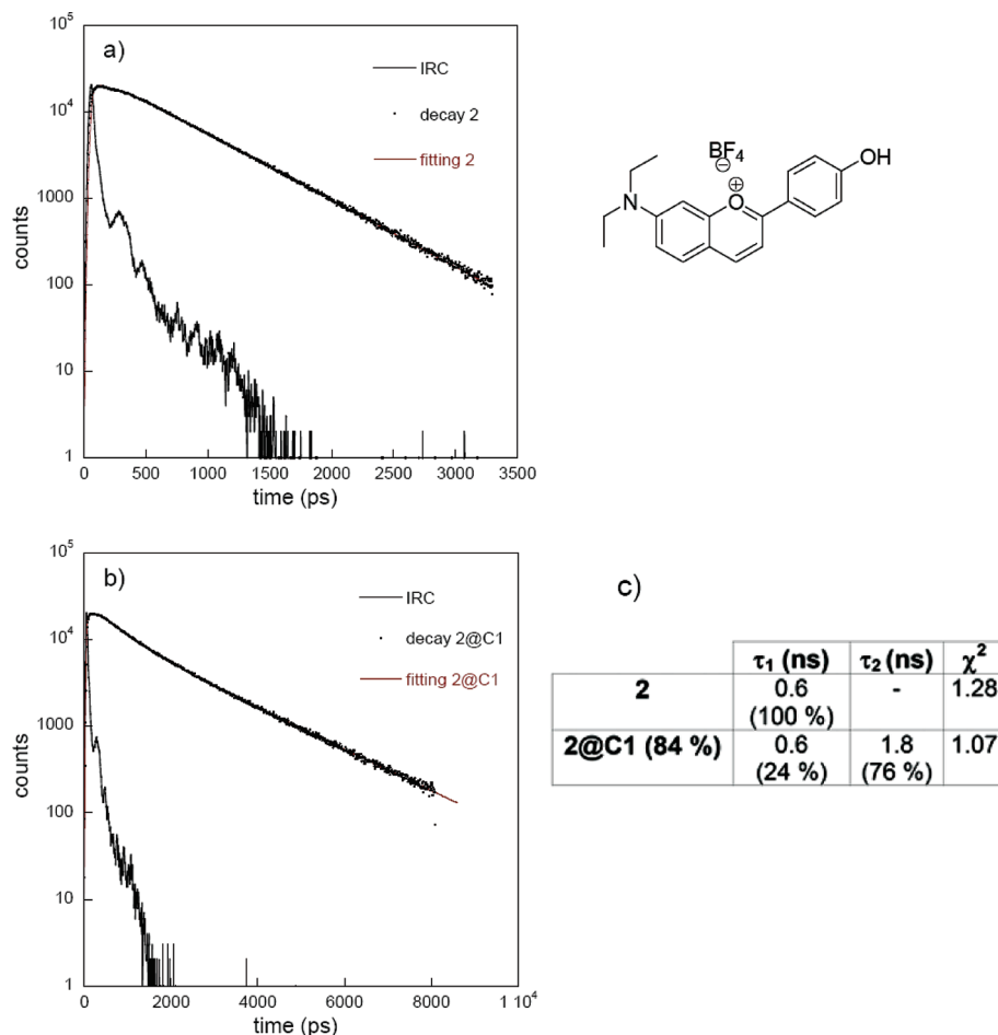
Figure 5. Fluorescence decays of flavylum 2 (a) and 2@C1 (84% complexation) (b) in methanol. Excitation at 390 nm, emission at 650 nm, scale 3.44 ps/channel for 2 , 8.4 ps/channel for 2@C1 . (c) Table with fitting parameters for flavylum salt 2 in the absence (lifetime 0.6 ns) and in presence of clip C1 (lifetime 1.8 ns).
