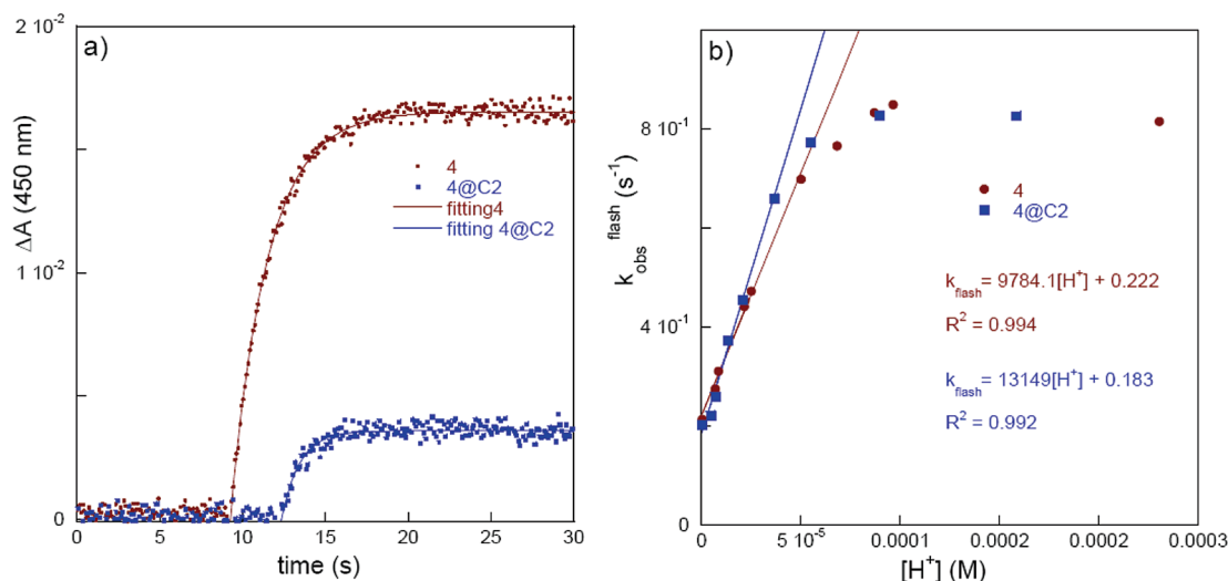
Figure 18. (a) Differential absorbance at 450 nm vs time in seconds in the absence (red, 4 , pH 4.66) and in presence of C2 (blue, 4@C2 , pH 4.06), [\text{4}] = 7.2 \times 10^{-6} \text{ M} , [\text{C2}] = 8.7 \times 10^{-5} \text{ M} . Fitting was obtained using an exponential function with k_{\text{flash}}^{\text{obs}} = 0.91 \text{ s}^{-1} in the presence of clip pH 4.06 and 0.45 \text{ s}^{-1} without clip pH 4.66. (b) Rates of flash photolysis vs [\text{H}^+] for 4 (red) and 4@C2 (blue). Linear regressions and obtained equations and correlation coefficients are shown.
