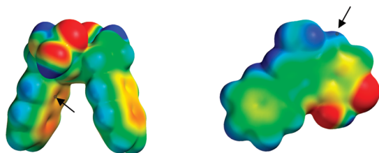
Figure 11. Electrostatic potential surface (EPS) calculated for clip C1 substituted by dihydrogen phosphate groups ( \text{OPO}(\text{OH})_2 instead of \text{OPO}_2(\text{OH})\text{Li}^+ ) (left) and quinoidal base 3A (right) by the use of density functional B3LYP/6-31G**//AM1 (implemented in SPARTAN) (ref 24). The color code ranges from -25 kcal/mol (red) to +25 kcal/mol (blue). The molecular electrostatic potential (MEP) was calculated at the marked position to be -19 kcal/mol at the clip naphthalene sidewalls and +18 kcal/mol at hydrogen atom 5-H of 3A .
