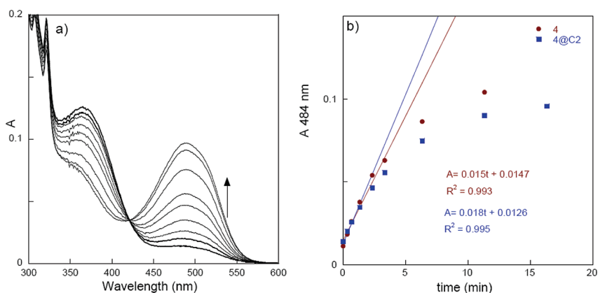
Figure 19. (a) Spectral modifications that occur upon irradiation at 390 nm of an aqueous solution of equilibrated [\text{4}] = 6.3 \times 10^{-6} \text{ M} at pH = 5.7 in presence of clip [\text{C2}] = 4.0 \times 10^{-5} \text{ M} . (b) Changes in absorbance at 484 nm in the absence (red circles, 4 ) and in presence of C2 (blue squares, 4@C2 ) with time.
