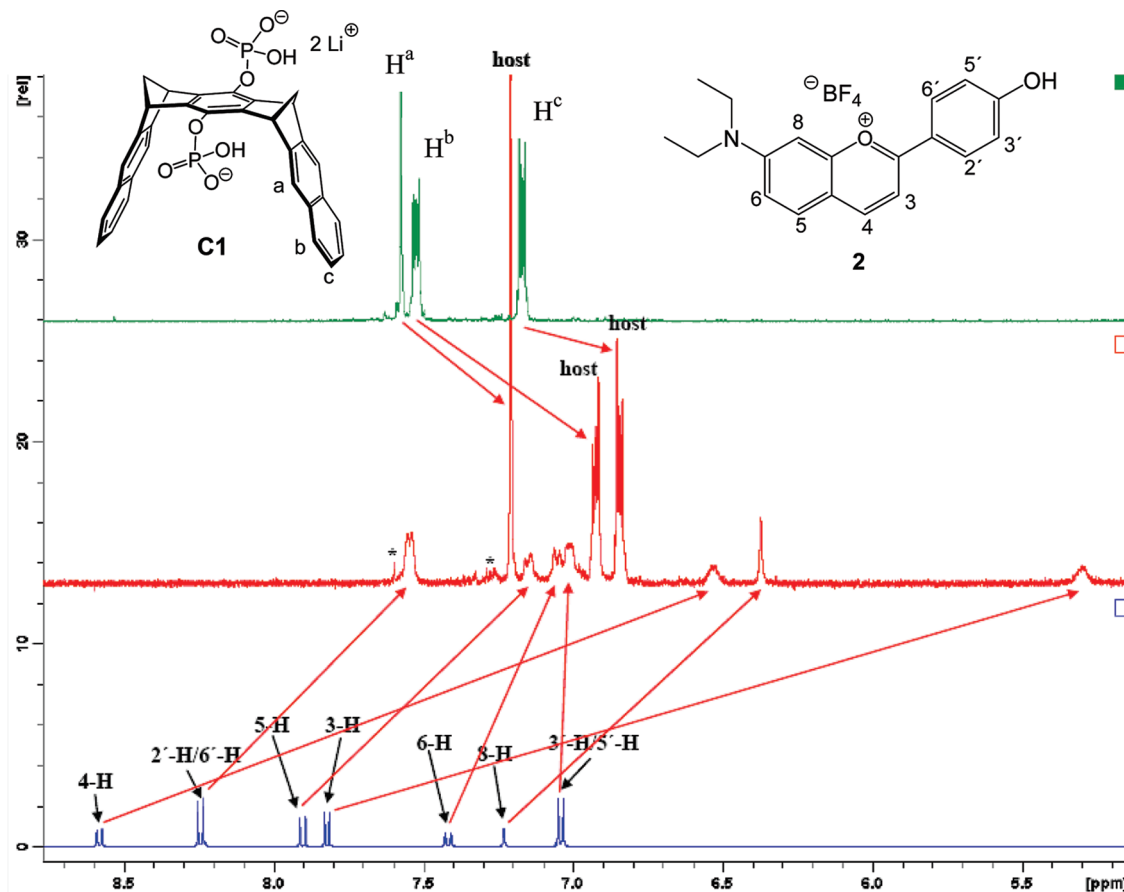
Figure 7. ^1\text{H} NMR spectra (500 MHz, \text{CD}_3\text{OD} , 25 ^\circ\text{C} ) of clip C1 (5.07 mM) (top), a mixture of C1 (1.53 mM) and flavylum salt 2 (1.50 mM) (middle), and flavylum salt 2 (1.50 mM) (bottom) (aromatic range); * impurities.
