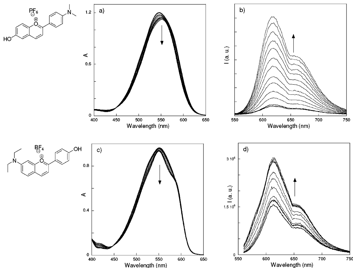
Figure 3. Spectral modifications observed upon addition of molecular clip, [C1] = 0\text{--}7 \times 10^{-4} M, to methanolic solutions of 4'-dimethylamino-6-hydroxyflavylium hexafluorophosphate, [1] = 1.92 \times 10^{-5} M, followed by absorption (a) and fluorescence emission (b) (2 nm slits, \lambda_{\text{exc}} = 545 nm) and to methanolic solutions of 7-diethylamino-4'-hydroxyflavylium hexafluorophosphate, [2] = 2.26 \times 10^{-5} M, followed by absorption (c) and fluorescence emission (d) (2 nm slits, \lambda_{\text{exc}} = 550 nm).
