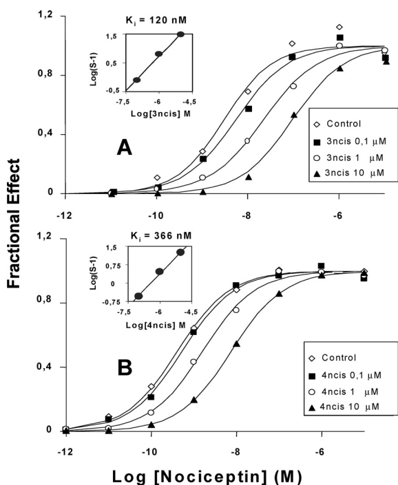
Fig. 5. Antagonism of Nociceptin-Mediated Activation of G_{a_o} Induced by Compounds 3n cis and 4n cis
