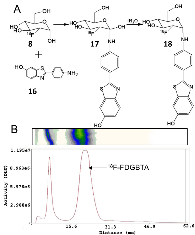
Figure 4. (A) Radiosynthesis of 18 F-FDGBTA ( 18 ) showing reaction of 18 F-FDG ( 8 ) with BTA ( 16 ) and subsequent dehydration of intermediate 17 . (B) Radio-TLC of 18 F-FDGBTA ( 18 ) reaction mixture, showing the presence of product.
