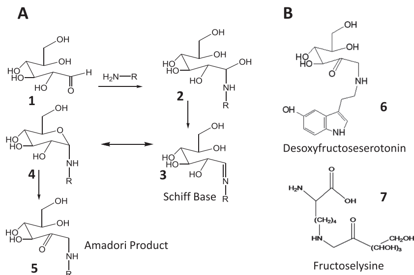
Figure 1. (A) Reaction scheme showing Maillard reaction of glucose (1) and substituted amine resulting in the formation of Schiff base (3) and subsequent isomerization to the Amadori product (5). (B) Example of Amadori products, desoxyfructoseserotonin (6), and fructoselysine (7).
