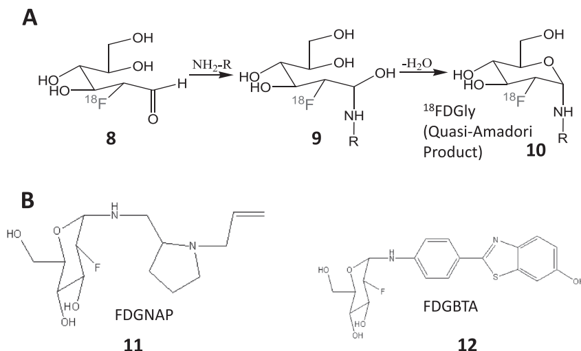
Figure 2. (A) Generic synthesis scheme of ^{18}\text{F} -FDG (8) with amines leading to the ^{18}\text{F} -FDGly (10), quasi-Amadori product. This is expected from reaction of ^{18}\text{F} -FDG with amines. (B) Two synthesized FDGly products are reported here: FDGNAP (11) and FDGBTA (12).
