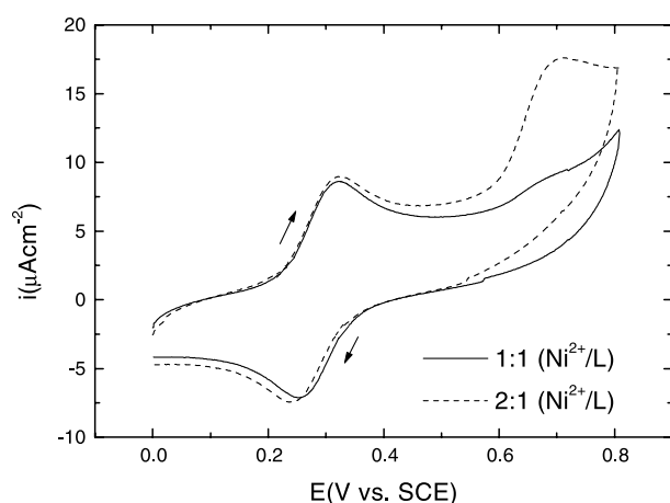
Fig. 4. Cyclic voltammograms of ligand 3 in the presence of \text{Ni}^{2+} ion.
