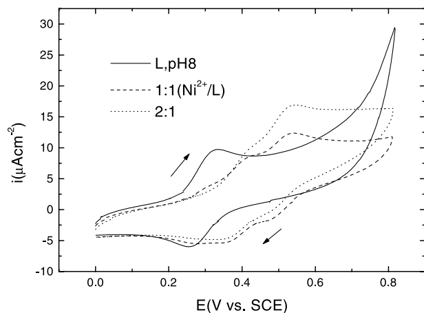
Fig. 5. Cyclic voltammograms of ligand 4 in the presence or absence of \text{Ni}^{2+} ion.
