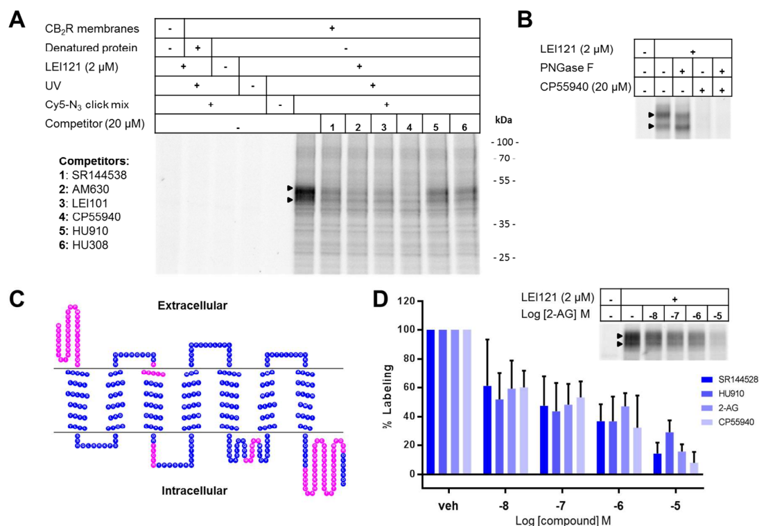
Figure 3: Validation of CB 2 R labeling by LEI121 in CB 2 R-overexpressing CHO cells. A) LEI121 labels displaceable bands (▶ = CB 2 R) specifically in CB 2 R-overexpressing membranes, not in wildtype CHO membranes, and only in presence of all necessary components (active protein, probe, UV-irradiation, ligation components). B) Addition of PNGase F shows a decrease of higher MW glycosylated CB 2 R bands, and an increase in full-length, probe-bound CB 2 R signal (~41 kDa). The gel shown is a representative result of three independent experiments. C) Isolation of CB 2 R was achieved in live CB 2 R-overexpressing cells by ligation with biotin-N 3 ( 15 ), followed by avidin enrichment, trypsinization and proteomics. CB 2 R peptides identified from 3 independent experiments are highlighted in magenta. D) Quantification of dose-dependent displacement of LEI121-labeled bands in SDS-PAGE experiments by different cannabinoid ligands. Results shown are the mean \pm SEM of 2 (CP55940 and 2-AG) or 3 (SR144528 and HU910) independent experiments. The inset shown is a representative gel of concentration-dependent displacement of LEI121 labeling by 2-AG (see also Figure S8 ).
