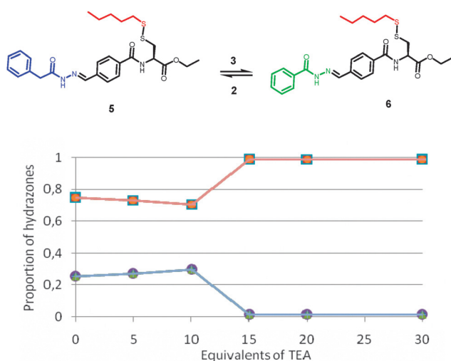
Fig. 1 Proportion of 5 (■) and 6 (●) after 24 h of reaction in chloroform in the presence of 15 equivalents of TFA and different amounts of TEA.
