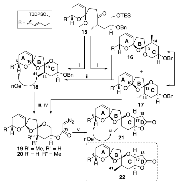
Scheme 3 (i) PPTS, THF, H 2 O, 40% 16 , 36% 17 ; (ii) CSA, hexanes, 42% 18 , 32% 16 , 7% 17 ; (iii) LiDBB, THF, -78 °C, 10 min; (iv) ClCOCH=N-NHTs, N,N -dimethylaniline, Et 3 N, CH 2 Cl 2 , 60% 19 over 2 steps, 65% 20 over 2 steps; (v) Rh 2 (4S)-(MPPIM) 4 , CH 2 Cl 2 , reflux, 12% 21 .
