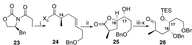
Scheme 4 (i) NaHMDs, ICH 2 CH=CHCH 2 CH 2 OBn, THF, 92%; (ii) AD mix β*, NaHCO 3 , t -BuOH, H 2 O, r.t., 4 : 1 d.r., 55%; (iii) TIPSOt, imid., DMF, 88%; (iv) LiBH 4 , MeOH, THF, 99%; (v) PivCl, DMAP, Et 3 N, CH 2 Cl 2 , 82%; (vi) BnBr, NaH, DMF; (vii) TBAF, THF, 24% over 2 steps; (viii) TESCl, DMAP, Et 3 N, CH 2 Cl 2 , 99%; (ix) LiBH 4 , MeOH, THF, 89%; (x) TPAP, NMO, CH 2 Cl 2 , mol. sieves, 95%.
