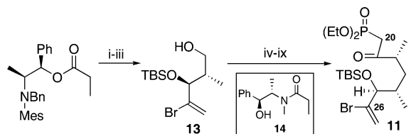
Scheme 2 (i) Cyx 2 BOTf, Et 3 N, 2-bromoacrolein, Et 2 O, 92%, 93 : 7 d.r.; (ii) TBSOTf, Et 3 N, DMAP, CH 2 Cl 2 , 62%; (iii) DIBAL-H, CH 2 Cl 2 , -78 °C, 86%; (iv) Ph 3 P, imid., I 2 , CH 2 Cl 2 , 88%; (v) LDA, LiCl, THF, 92%; (vi) LDA, BH 3 ·NH 3 , THF, 84%; (vii) TPAP, NMO, CH 2 Cl 2 , mol. sieves; (viii) Me(O)P(OEt) 2 , n -BuLi, THF; (ix) PDC, DMF, mol. sieves, 53% over 3 steps.
