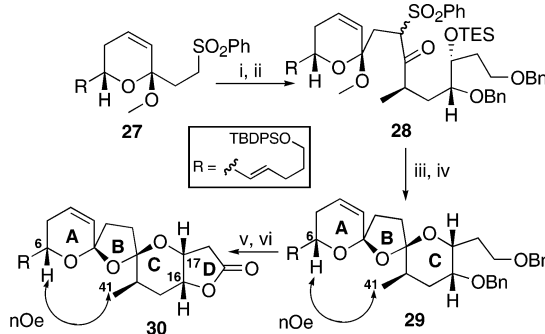
Scheme 5 (i) 27 , LDA, THF, then 26 , -78 °C; (ii) TPAP, NMO, CH 2 Cl 2 , mol. sieves, 66% yield over 2 steps; (iii) Na/Hg, Na 2 HPO 4 , THF, H 2 O, 82%; (iv) PPTS, THF, H 2 O, 50%; (v) LiDBB, THF, -78 °C; (vi) TPAP, NMO, CH 2 Cl 2 , mol. sieves, 73% over 2 steps.
