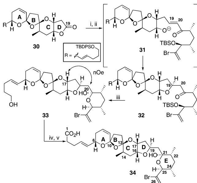
Scheme 6 (i) DIBAL-H, CH 2 Cl 2 , -78 °C, 78%; (ii) 11 , KHMDS, THF, -78 °C to r.t., 45%; (iii) TBAF, THF, 57%; (iv) TPAP, NMO, CH 2 Cl 2 , mol. sieves, 68%; (v) NaClO 2 , t -BuOH, H 2 O, 2-methyl-2-butene, 60%.
