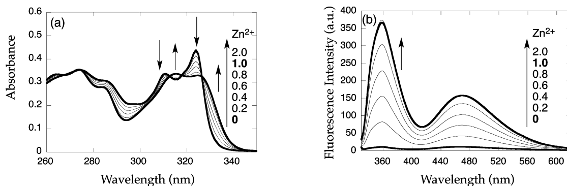
Figure 2. (a) UV-vis absorption and (b) fluorescence ( \lambda_{\text{ex}} = 324 nm) spectra of 34 \mu\text{M} 1-isoTQA in DMF/H 2 O (1:1) at 25 °C in the presence of various concentration of Zn 2+ ranging from 0 to 68 \mu\text{M} .
