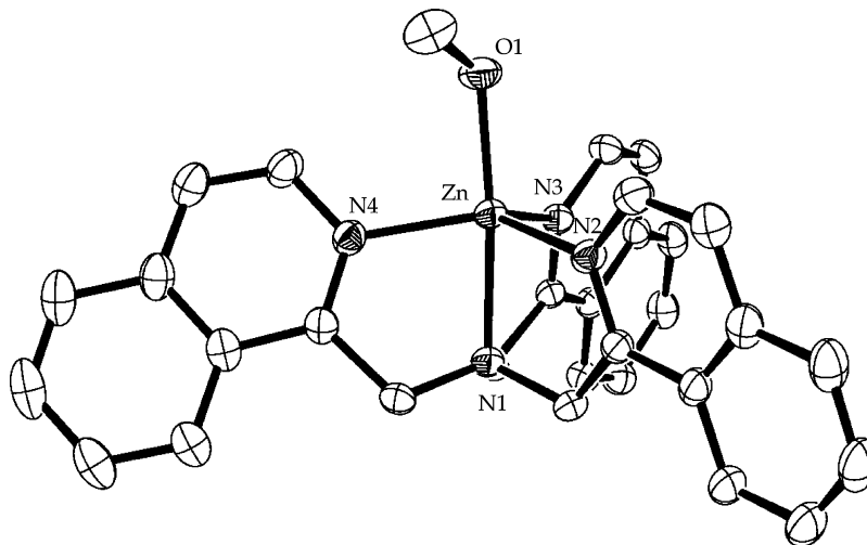
Figure 4. ORTEP plot for [Zn(1-isoTQA)(CH 3 OH)](ClO 4 ) 2 ·2CH 3 OH in 50% probability. Atoms of counteranions, hydrogen, and solvents were omitted for clarity.
