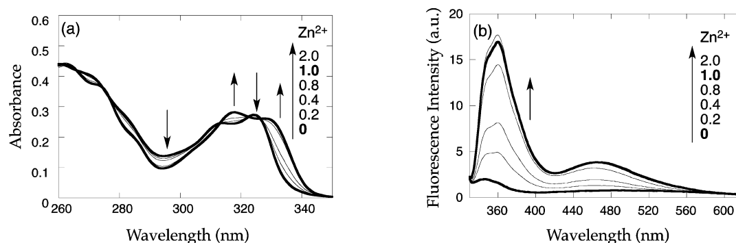
Figure 3. (a) UV-vis absorption and (b) fluorescence ( \lambda_{\text{ex}} = 324 nm) spectra of 34 \mu\text{M} 3-isoTQA in DMF/H 2 O (1:1) at 25 °C in the presence of various concentration of Zn 2+ ranging from 0 to 68 \mu\text{M} .
