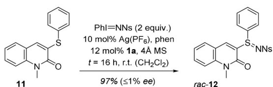
Scheme 7. Ag-catalyzed sulfimidation of 2-quinolone 11 under the conditions previously applied to substrates 3 and 5 (60 μmol scale, substrate concentration c = 10 mM). Within the limits of error, product 12 was formed as the racemate ( rac - 12 ).
