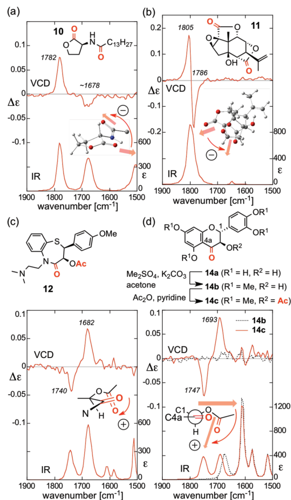
Figure 3. VCD (top) and IR (bottom) spectra and arrangement of two carbonyl chromophores of natural products and drugs. The spectra were measured for 2 and 90 min, respectively, in CDCl 3 ( l = 100 \mu m) at a concentration of 0.075 M ( 10 and 12 ) or 0.05 M ( 11 and 14 ). Each spectrum was corrected by a solvent spectrum obtained under identical measurement conditions. Each wavenumber at the extrema is labeled in italic . The alkyl chain in the model of 10 is omitted for clarity. The derivatization scheme of 14 is shown in (d).
