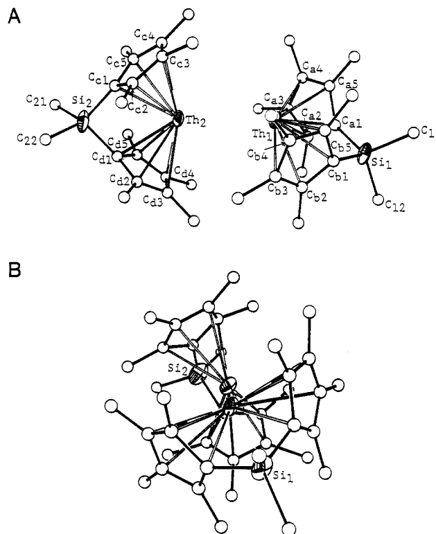
Figure 2. Two views of the molecular structure of [(CH 3 ) 2 Si[(CH 3 ) 4 C 5 ] 2 ThH 2 ] ( 3 ). Thorium and silicon atoms are represented by thermal vibration ellipsoids drawn to encompass 50% of the electron density; carbon atoms are represented by open spheres. Hydrogen atoms were not located.
