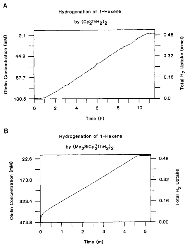
Figure 3. Plots of hydrogen uptake (in mmol) as a function of time during the hydrogenation of 1-hexene at 1.0 atm of H 2 pressure by the following organothorium catalysts in heptane: A, (\text{Cp}'_2\text{ThH}_2)_2 , 13.33 mM in Th; B, (\text{Me}_2\text{SiCp}''_2\text{ThH}_2)_2 ( 3 ), 9.39 mM in Th. Both plots illustrate the zero-order dependence of the rate on olefin concentration.
