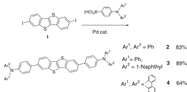
Scheme 1. Synthesis of DPh-BTBT derivatives.
