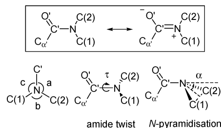
FIGURE 4. Structural parameters reflecting amide distortion.
