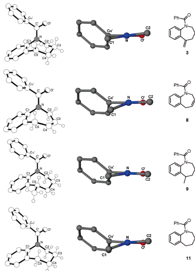
FIGURE 3. Molecular structures of benzazepines 3 , 8 , 9 and 11 (with chemical numbering scheme) and accompanying ball-and-stick models of the views along the N–C' axes, illustrating the nature of the amide twist.
