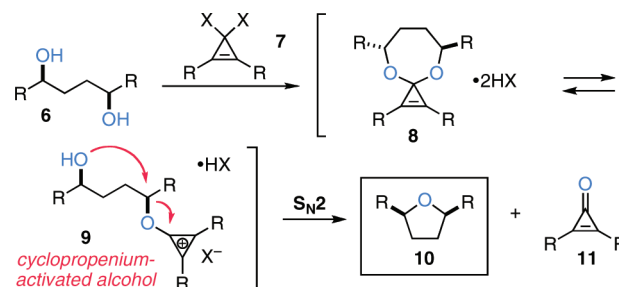
Figure 2. Mechanistic design for cyclopropenium ion mediated cyclization of diols to form cyclic ethers.
