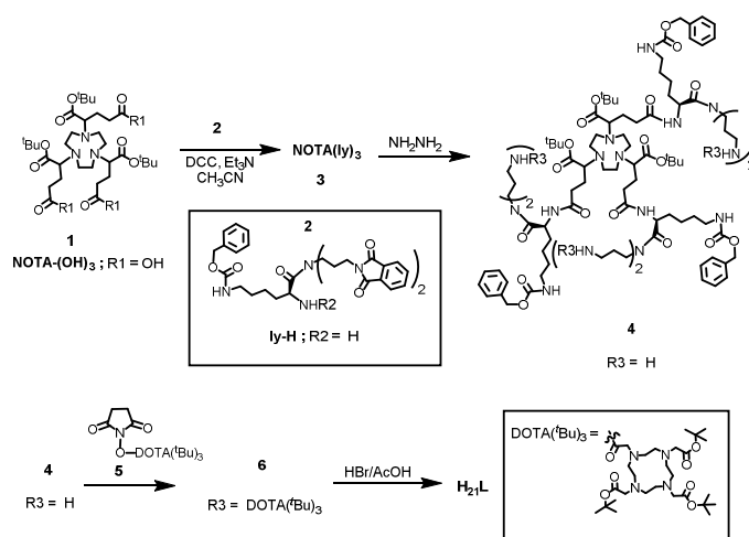
Scheme 1. Synthetic route to ligand H 21 L
