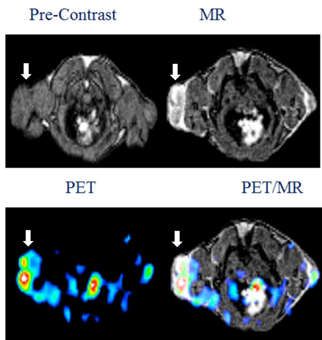
Figure 4. Representative MRI (upper panel), PET (lower panel – left), and fused PET/MR (lower panel – right) images of U87MG tumor xenograft in SCID mice at 1 h post injection of Gd 6 L[PEG 12 c(RGDyK)] 3 68 Ga. The white arrow indicates the tumor site.
