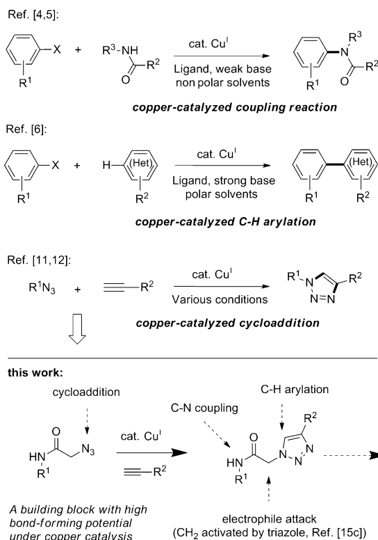
Scheme 1. Merging of copper-mediated cross-coupling and cycloaddition reactions by a “click-and-activate” protocol.
