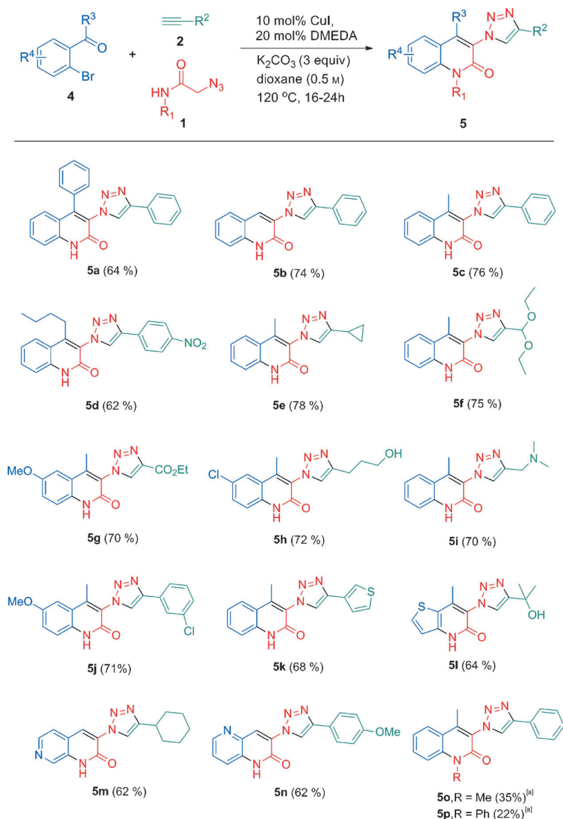
Scheme 4. Synthesis of 3-triazolylquinolinones 5 by the copper-catalyzed, three-component condensation of a 2-azidoacetamide 1 , an alkyne 2 , and an o -acyl aryl bromide 4 . [a] Cs_2CO_3 /toluene (120 °C, 36 h) was used instead of K_2CO_3 /dioxane.
