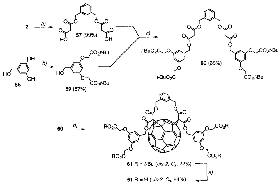
Scheme 11. Preparation of Tetraacid 51
