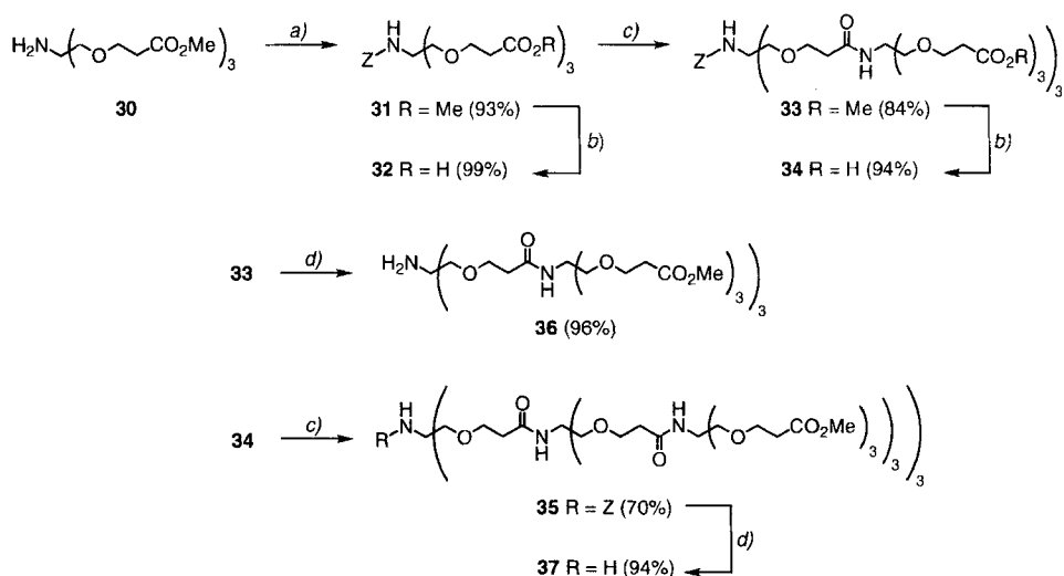
Scheme 6. Synthesis of Dendrons 36 and 37
