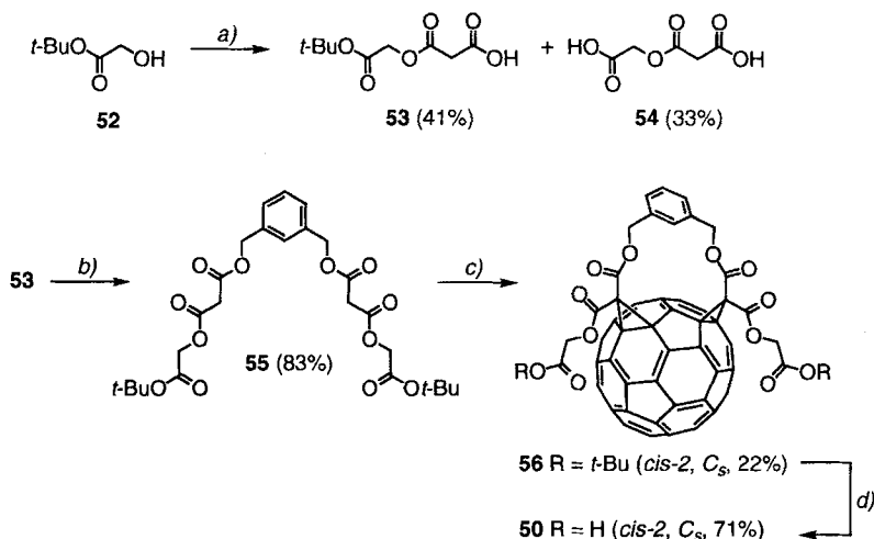
Scheme 10. Preparation of Diacid 50
