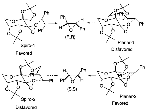
Figure 2. The spiro and planar transition states for trans -stilbene epoxidation catalyzed by ketone 3 .
