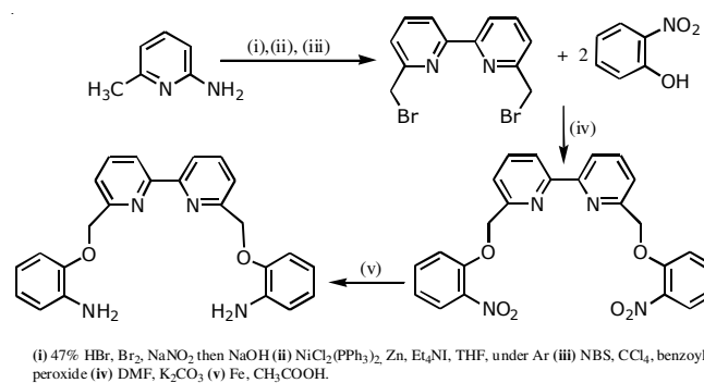
Scheme-I: Synthetic route for diamine compound, 6,6'-bis(2-aminophenoxy)methyl-2,2'-bipyridine
