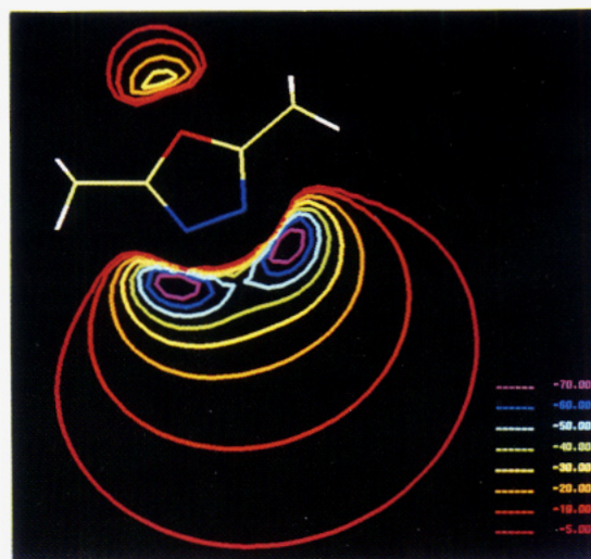
2,5-dimethyl-1,3,4-oxadiazole
