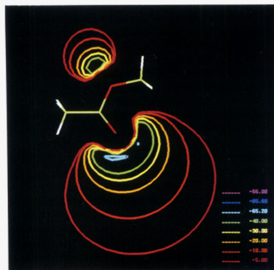
methyl acetate
