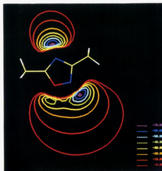
3,5-dimethyl-1,2,4-oxadiazole
