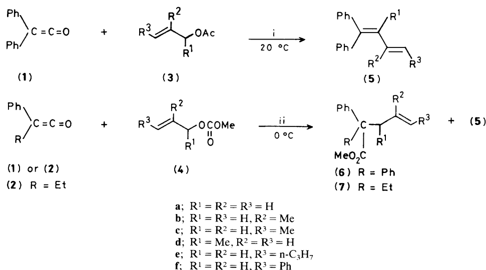
Scheme 1. Reagents: i, \text{Pd}(\text{PPh}_3)_4 , in benzene, 1–20 h; ii, \text{Pd}(\text{PPh}_3)_4 , in DMF, 0.5 h, -\text{CO}_2 .
