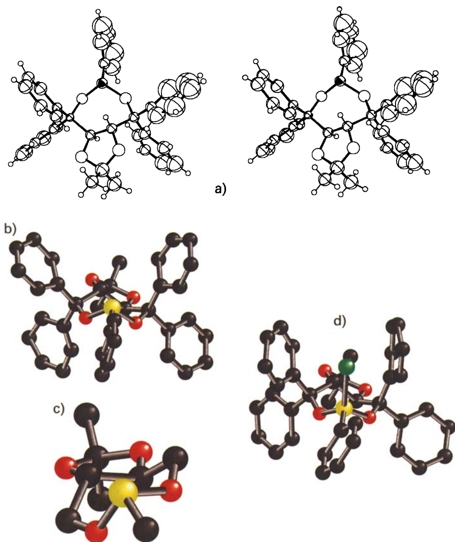
Figure. Structure of the phosphonite 2b (C: black, O: red, P: yellow, Rh: green). a) ORTEP [22] stereoview of a single molecule of the crystal structure of 2b . Vibrational ellipsoids are drawn at the 40% level (because of an exceptionally long unit cell axis of 116 Å, only isotropic refinement was possible, see Exper. Part ). b) Projection showing the quasi -axial and quasi -equatorial disposition of the Ph groups in 2b . c) Chair-type conformation of the seven-membered ring in 2b . d) Modelling of a Rh complex of 2b with SYBYL [22]. In the crystal structure, the space of the Rh-atom is occupied by a Ph ring of another molecule. The Rh-atom was attached to the P-atom at a distance of 2.2 Å (mean value of Rh–P fragments found in the Cambridge Data Base [23]). For the relaxation of the constructed complex, the Rh–P distance was fixed and only van der Waals repulsion between the Rh-atom and the rest of the molecule contributed to the energy calculation. Projections b–d were generated with PLUTO78 [23] and SYBYL [22].
