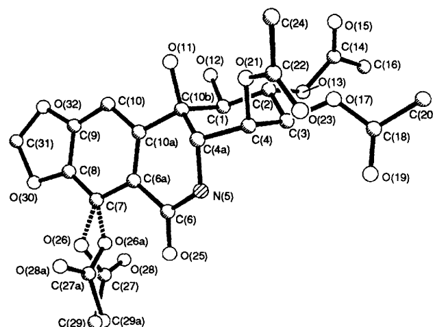
Fig. 1 X-ray molecular structure of 2,3,4,7-tetraacetoxy-10b- R -hydroxypancratistatin 5 (less H atoms) depicting the two C-7 acetate rotamers
