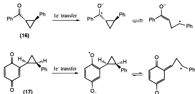
Scheme 3. Other Examples of Cyclopropane Isomerization Reactions Occurring via Free Radical-Induced Reversible Ring Openings (See ref 21 and 22)
