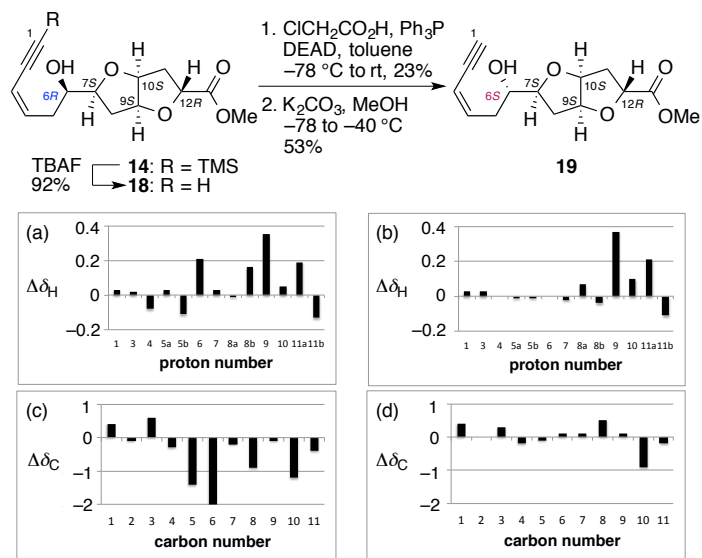
Figure 4. Chemical shift differences between the synthetic compound ( 18 or 19 ) and the natural laurenidificin. The x -axis represents proton or carbon number. The y -axis shows chemical shift differences in ppm. (a) \Delta\delta_{\text{H}} = (\mathbf{18}) - (\text{natural product}) . (b) \Delta\delta_{\text{H}} = (\mathbf{19}) - (\text{natural product}) . (c) \Delta\delta_{\text{C}} = (\mathbf{18}) - (\text{natural product}) . (d) \Delta\delta_{\text{C}} = (\mathbf{19}) - (\text{natural product}) .
