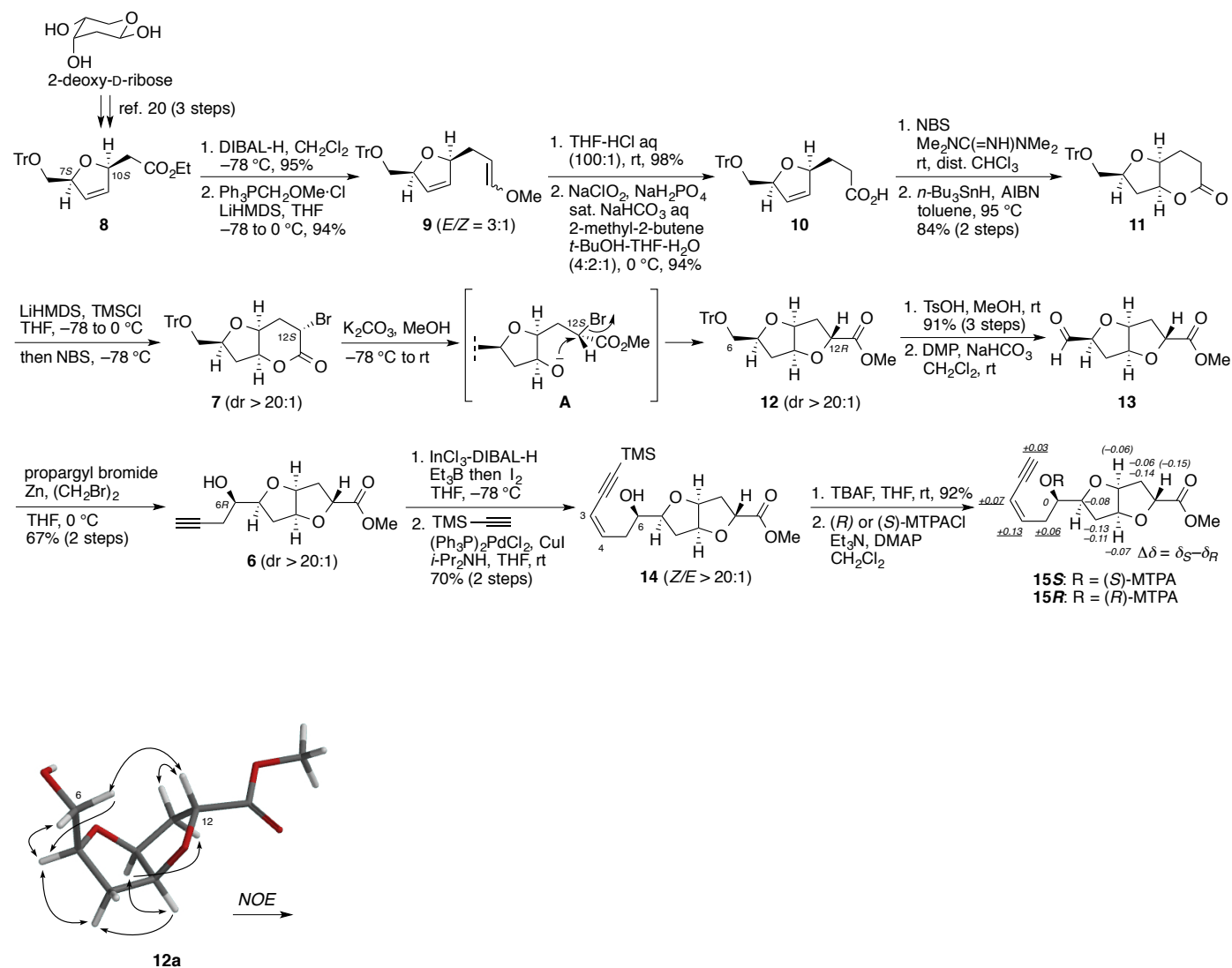
Figure 2. NOE correlations for 12a . The energy-minimized structure was obtained by the molecular mechanics calculation with MMFF force field.
