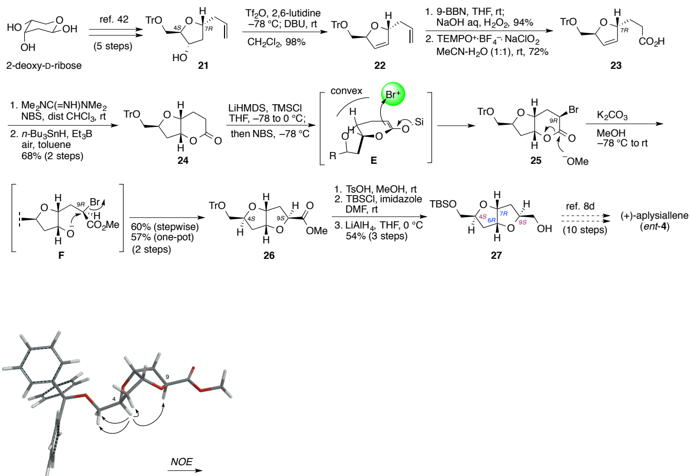
Figure 5. NOE correlations for 26 . The energy-minimized structure was obtained by the molecular mechanics calculation with MMFF force field.
