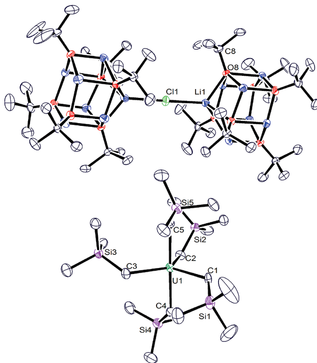
Figure 1. ORTEP diagram of [\text{Li}_4(\text{O}'\text{Bu})_{12}\text{Cl}][\text{U}(\text{CH}_2\text{SiMe}_3)_5] ( 1 ) with 30% probability ellipsoids. Selected bond lengths (Å) and angles (deg): \text{U1}-\text{C1} = 2.451(6) , \text{U1}-\text{C2} = 2.445(6) , \text{U1}-\text{C3} = 2.461(6) , \text{U1}-\text{C4} = 2.485(6) , \text{U1}-\text{C5} = 2.463(5) , \text{U1}-\text{C1}-\text{Si1} = 126.2(3) , \text{U1}-\text{C2}-\text{Si2} = 127.6(3) , \text{U1}-\text{C3}-\text{Si3} = 125.7(3) , \text{U1}-\text{C4}-\text{Si4} = 128.9(3) , \text{U1}-\text{C5}-\text{Si5} = 130.6(3) , \text{C1}-\text{U1}-\text{C2} = 112.8(2) , \text{C1}-\text{U1}-\text{C3} = 122.9(2) , \text{C2}-\text{U1}-\text{C3} = 123.9(2) , \text{C1}-\text{U1}-\text{C4} = 86.9(2) , \text{C1}-\text{U1}-\text{C5} = 92.5(2) .
