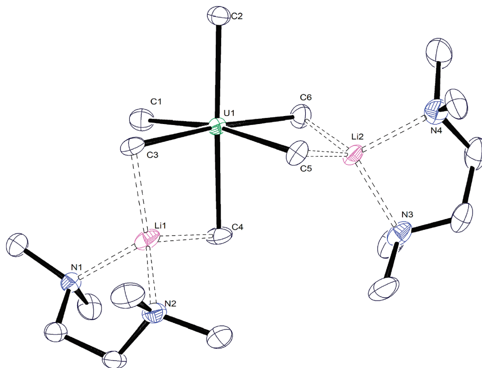
Figure 3. ORTEP diagram of [\text{Li}(\text{TMEDA})]_2[\text{UMe}_6] ( 4 ) with 30% probability. Selected bond lengths (Å) and angles (deg): \text{U1}-\text{C1} = 2.48(1) , \text{U1}-\text{C2} = 2.483(9) , \text{U1}-\text{C3} = 2.564(9) , \text{U1}-\text{C4} = 2.557(9) , \text{U1}-\text{C5} = 2.600(9) , \text{U1}-\text{C6} = 2.55(1) , \text{Li1}-\text{C3} = 2.21(2) , \text{Li1}-\text{C4} = 2.19(2) , \text{Li2}-\text{C5} = 2.18(2) , \text{Li2}-\text{C6} = 2.26(2) , \text{C1}-\text{U1}-\text{C2} = 94.8(3) , \text{C1}-\text{U1}-\text{C3} = 89.4(3) , \text{C1}-\text{U1}-\text{C4} = 85.9(3) , \text{C1}-\text{U1}-\text{C5} = 170.1(3) , \text{C1}-\text{U1}-\text{C6} = 96.4(3) , \text{C2}-\text{U1}-\text{C5} = 93.8(3) .
