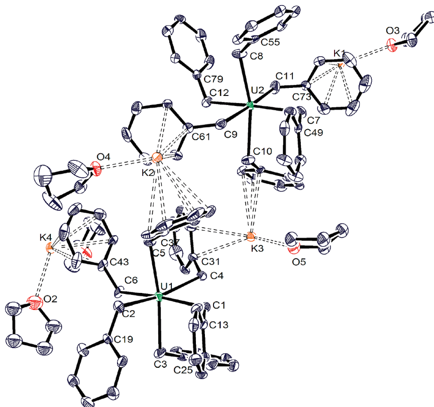
Figure 4. ORTEP diagram of the asymmetric unit in crystals of \{[\text{K}(\text{THF})_3][\text{K}(\text{THF})_2][\text{U}(\text{C}_6\text{H}_5)_6]_2\}_x ( 5 ) with 30% probability ellipsoids. Selected bond lengths (Å) and angles (deg): U2–C7 = 2.53(2), U2–C8 = 2.50(2), U2–C9 = 2.56(2), U2–C10 = 2.54(2), U2–C11 = 2.57(2), U2–C12 = 2.53(2), K1–C73 = 3.17(2), K1–C74 = 3.27(2), K1–C77 = 3.23(2), K1–C78 = 3.12(2), K2–C61 = 3.16(2), K2–C62 = 3.28(2), K2–C65 = 3.35(2), K2–C66 = 3.17(2), U2–C7–C49 = 111(1), U2–C8–C55 = 124(1), U2–C9–C61 = 117(1), U2–C10–C67 = 121(1), U2–C11–C73 = 109(1), U2–C12–C79 = 122(1), C7–U2–C8 = 97.6(7), C8–U2–C9 = 85.7(6), C8–U2–C10 = 164.6(7), C8–U2–C11 = 93.7(7), C8–U2–C12 = 89.1(6).
