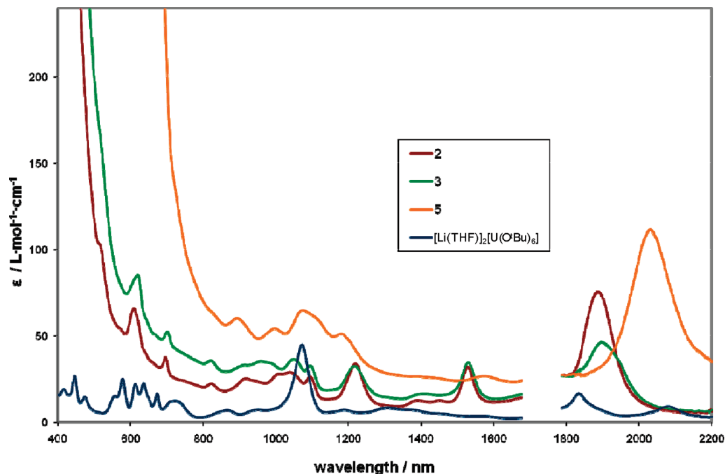
Figure 5. Room temperature NIR absorption spectra for 2 (3.20 mM, THF), 3 (5.22 mM, THF), 5 (3.30 mM, THF), and [\text{Li}(\text{THF})_2][\text{U}(\text{O}^i\text{Bu})_6] (9.51 mM, THF).
