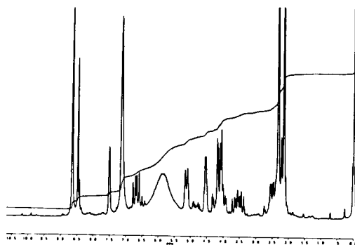
^1\text{H} -nmr of 30 in DMSO- d_6
