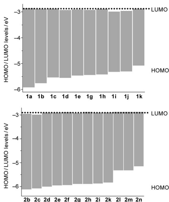
Figure 5. HOMO/LUMO energy levels calculated from the redox potentials of 1a–e,g–k and 2b–i,k–n .
