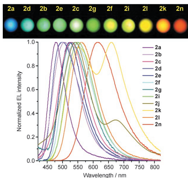
Figure 7. The OLEDs fabricated by using 2a–g,i,l,n and the corresponding EL spectra confirm effective blue-to-red emission tuning in the solid state.
