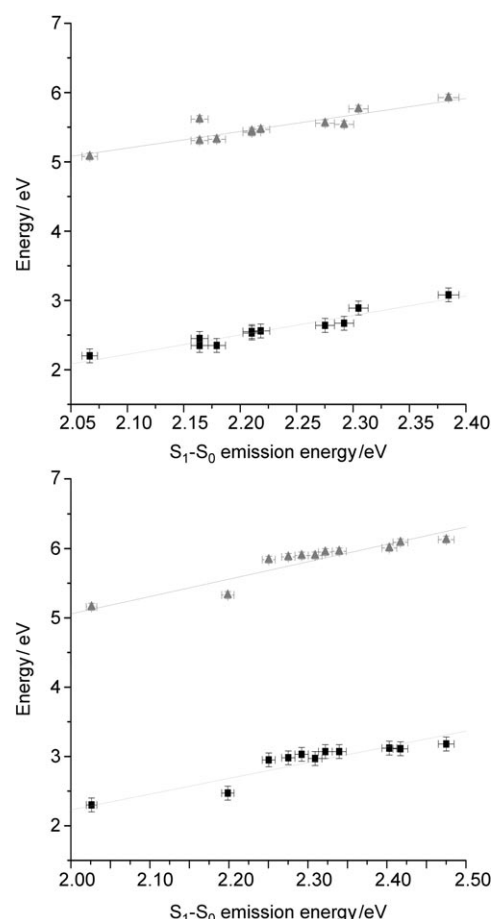
Figure 6. HOMO–LUMO gap (■) and HOMO level (▲) for 1a–k and 2a–n as a function of the fluorescence emission energy.
