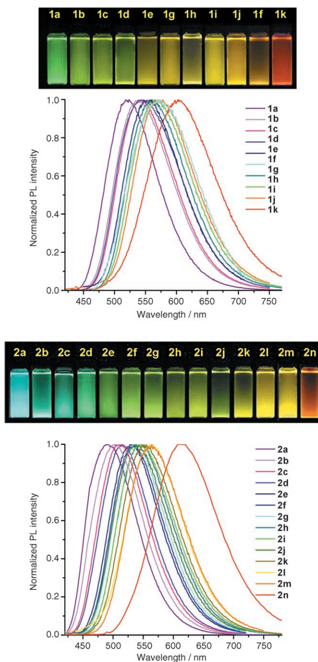
Figure 2. Emission of complexes 1a–k and 2a–n upon illumination with black light and the corresponding fluorescence spectra of complexes.
