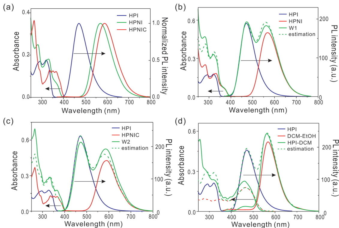
Figure 3. Optical properties of synthesized molecules in solution (CHCl 3 , c = 1 \times 10^{-5} M) at room temperature. (a) Absorption (Abs) and normalized photoluminescence (PL) of HPI (blue), HPNI (green), and HPNIC (red). (b) Abs and PL (excitation at 346 nm) spectra of HPI (blue), HPNI (red), and W1 (green solid line). The green dashed line indicates the expected spectrum of W1 as a superposition of HPI and HPNI (see text). (c) Abs and PL (excitation at 345 nm) spectra of HPI (blue), HPNIC (red), and W2 (green solid line). The green dashed line indicates the expected spectrum of W2 as a superposition of HPI and HPNIC. (d) Abs and PL (excitation at 345 nm) spectra of HPI (blue), DCM-EtOH (red), HPI-DCM (green solid line), and the expectation (green dashed line).
