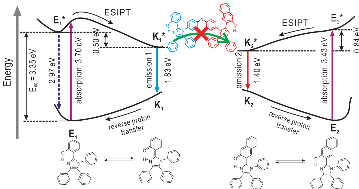
Figure 2. Diagram of the ESIPT process in the white-light-emitting molecular dyad. Calculated energy level in W1, with the HPI moiety on the left and HPNI on the right, according to TD-DFT calculations.
