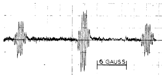
Figure 2. First-derivative esr spectrum of bicyclo[3.2.0]heptane-6,7-semidione ( 4 ) in DMSO solution at 25°, K + gegenion.
