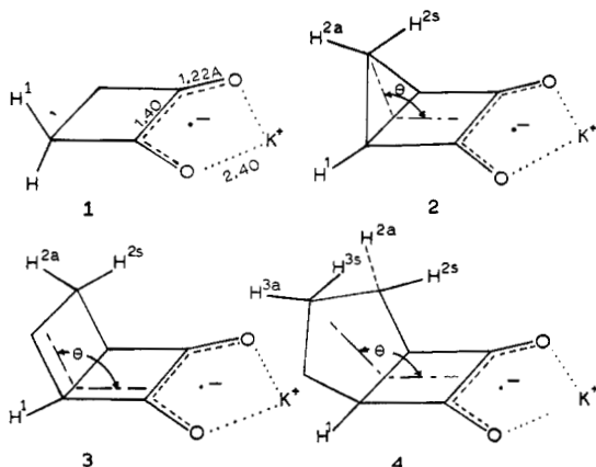
Figure 1. Geometry and numbering of cyclobutanesemidiones for MO calculations. All carbon-carbon single bonds were 1.54 Å, all carbon-hydrogen bonds 1.09 Å, and all H-C-H angles were taken as 111°. All rings were assumed to be planar. The methylene and methine hydrogen atoms were placed so that for a given group all H-C-C angles were equal.
