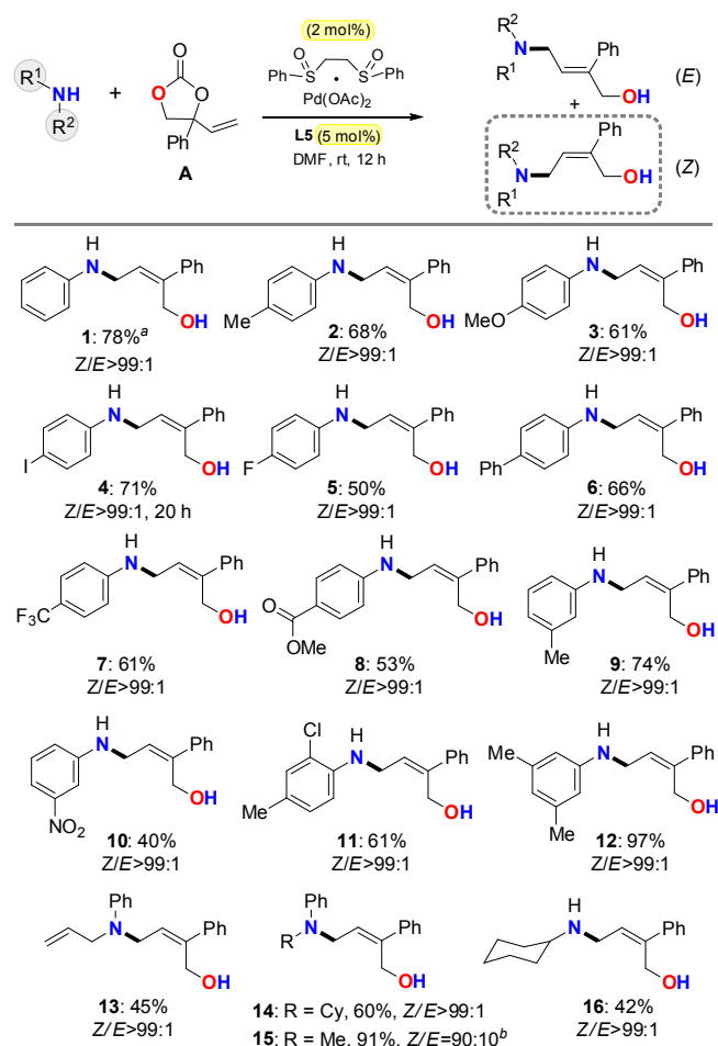
Figure 1. Scope in amine reaction partners: 0.2 mmol carbonate A used unless stated otherwise, 1.5 eq. of amine, rt, 12 h, open to air: No branched allylic amine formation could be observed. a 6 mmol scale. b 3 mmol scale.
