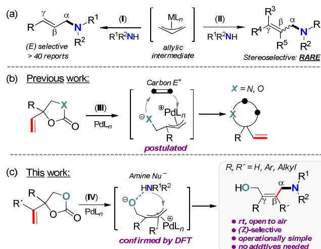
Scheme 1. Metal Catalyzed Allylic Chemistry for various Transformations.
