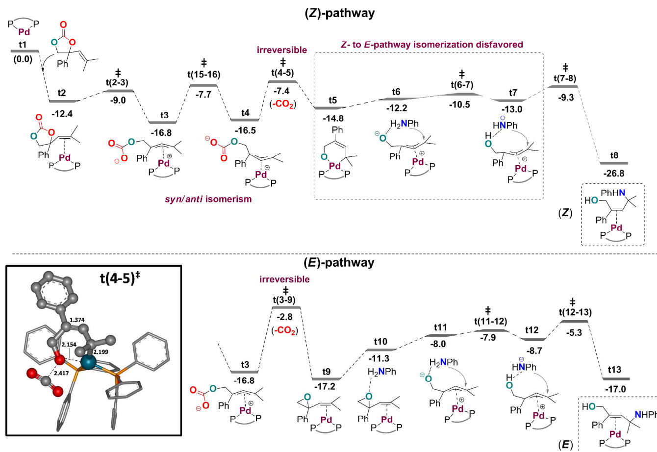
Figure 8. Computed free energy profile (in kcal/mol) for the synthesis of allylic amine product 40 reported in Figure 4. The structure of the transition state leading to t5 (i.e., t(4-5)^\ddagger ) is shown in the inset with selected calculated bond lengths.
