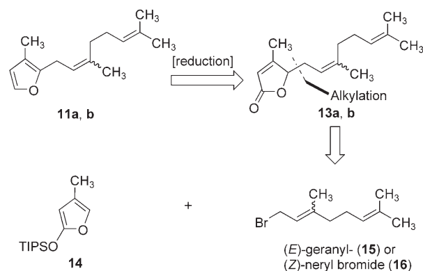
Scheme 3. Retrosynthetic analysis of furans 11a and 11b , precursors for the proposed biomimetic cascade sequence. TIPSO = triisopropylsilyl.
