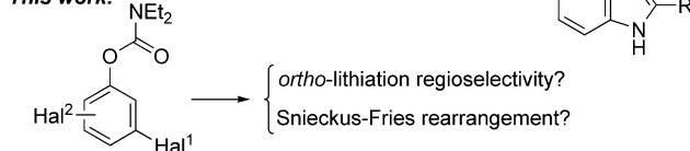
Scheme 1. Regioselectivity in the ortho -lithiation of O -halo-functionalized N,N -diethylcarbamates.
