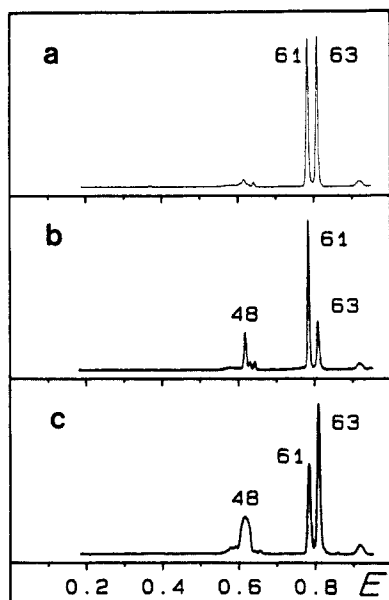
Figure 1. DADI spectra of the electron-impact-induced molecular ions of (a) DMSO (4), (b) aci -DMSO (5), and (c) methyl methanesulfonate (6).
