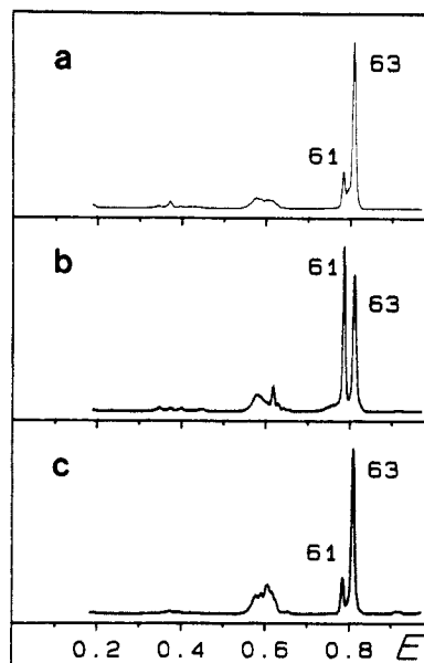
Figure 2. CA mass spectra of the electron-impact-induced molecular ions of (a) DMSO (4), (b) aci -DMSO (5), and (c) methyl methanesulfonate (6).
