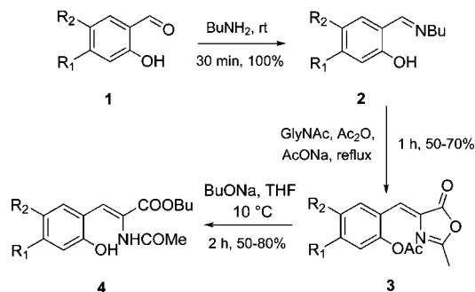
Scheme 1. Syntheses of Caged Model Alcohols cA ( 4a–c )
