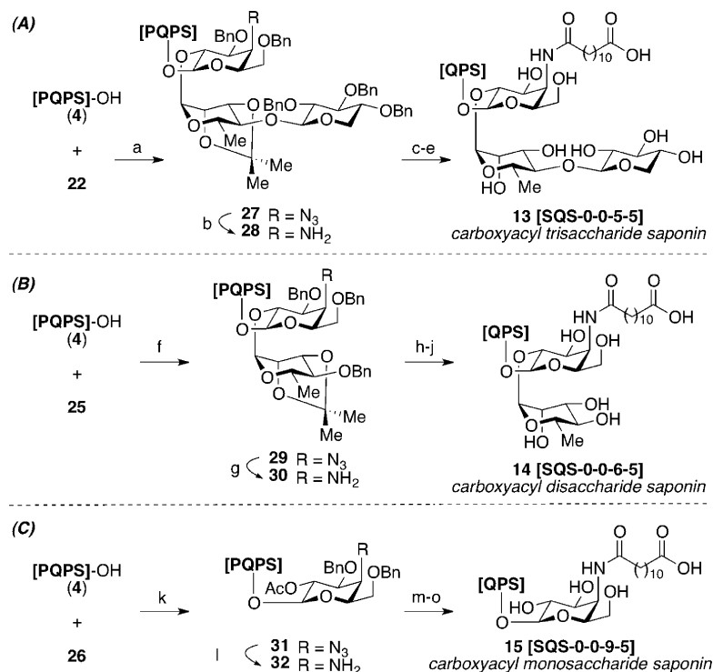
Scheme 4. Synthesis of Truncated Linear Tetrasaccharide Domain Variants 13–15 a
