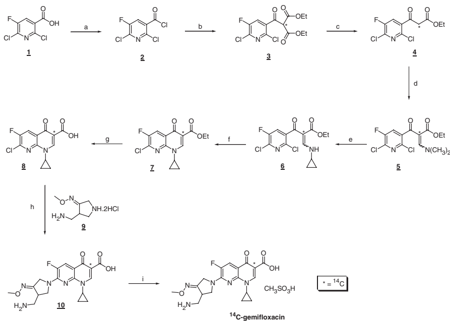
Scheme 2. Synthesis of ^{14}\text{C} -gemifloxacin: (a) \text{SOCl}_2 , cat. DMF, benzene, 110^\circ\text{C} , 3 h; (b) [2- ^{14}\text{C} ]diethyl malonate, magnesium ethoxide, diethyl ether, rt, 2 h; (c) p -TsOH, \text{H}_2\text{O} , 100\text{--}120^\circ\text{C} , 3 h; (d) DMFDA, \text{Ac}_2\text{O} , \text{CH}_2\text{Cl}_2 , rt, 2 h; (e) cyclopropyl amine, EtOH, rt, 1 h; (f) \text{K}_2\text{CO}_3 , DMF, 90^\circ\text{C} , 2 h; (g) c-HCl, AcOH, 120^\circ\text{C} , 4 h; (h) DBU, \text{CH}_3\text{CN} , rt, 22 h; (i) \text{CH}_3\text{SO}_3\text{H} , \text{CH}_2\text{Cl}_2/\text{EtOH} (7/3), 0^\circ\text{C} , 1 h
