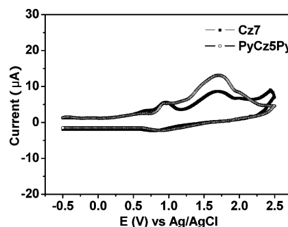
FIGURE 6. Cyclic voltammograms of Cz7 and PyCz5Py (0.5 mM) in 0.1 M Bu_4NPF_6-CH_2Cl_2 , scan rate 100 mV/s.
