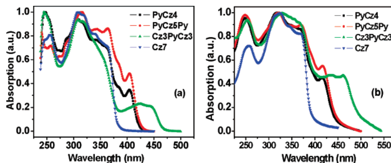
FIGURE 1. UV-vis absorption spectra of some compounds in THF (a) and in thin neat film (b).
