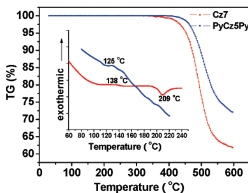
FIGURE 5. TGA and DSC (inset) thermograms of Cz7 and PyCz5Py in N_2 at a heating rate of 10 °C/min.
