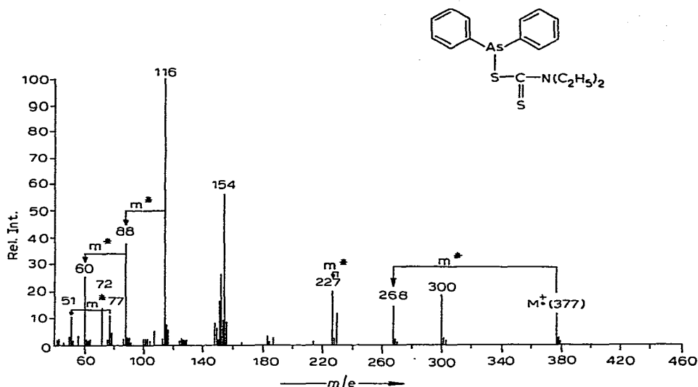
Fig. 3. Mass spectrum of S-diphenylarsino-N,N-diethyldithiocarbamate.
