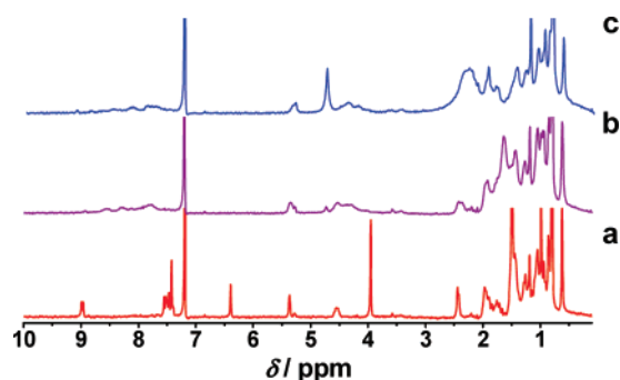
FIGURE 7. ^1\text{H} NMR spectra of the dye 3d in \text{CDCl}_3 with increasing concentration of \text{Zn}^{2+} in \text{CD}_3\text{CN} . The mole ratio of [\text{Zn}^{2+}] to [\text{3d}] is 0 (a), 0.25 (b), and 0.5 (c).
