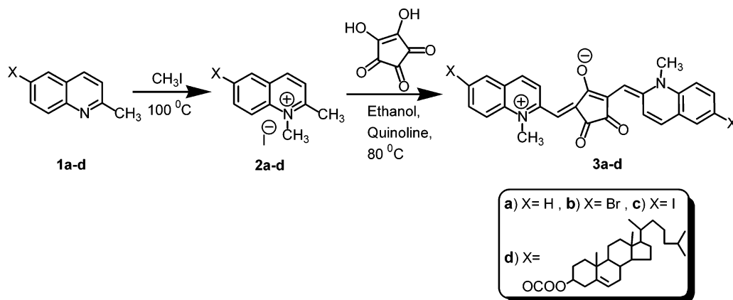
SCHEME 1. Synthesis of Croconaine Dyes 3a–d
