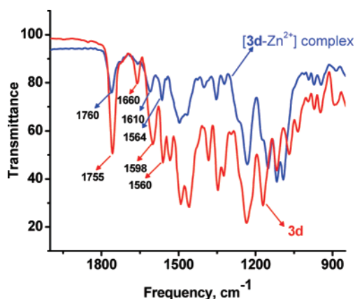
FIGURE 8. IR spectra of the croconaine dye 3d and the [\text{3d-Zn}^{2+}] complex.
