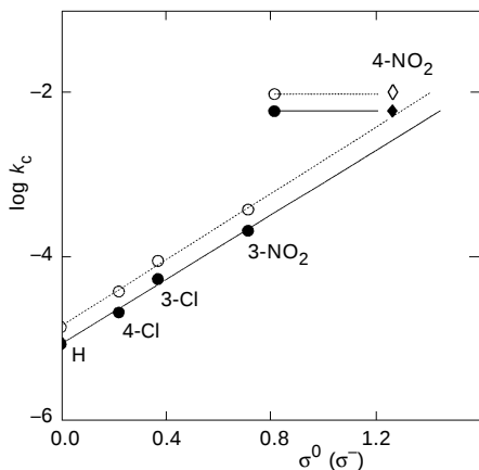
FIG. 1 Dependence of logarithms of cyclization rate constants of substituted phenyl N -(2-hydroxybenzyl)carbamates (●) and substituted phenyl N -(2-hydroxybenzyl)- N -methylcarbamates (○) on \sigma^0 constants in dioxane at 110 °C. For 4-nitrophenyl N -(2-hydroxybenzyl)carbamate (◆) and 4-nitrophenyl N -(2-hydroxybenzyl)- N -methylcarbamate (◇) on \sigma^- constant in dioxane at 110 °C
