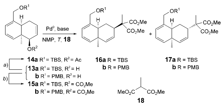
Scheme 3. Diastereoselectivities in the Pd-Catalyzed Allylic Alkylation
