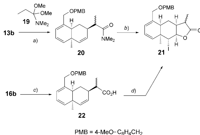
Scheme 4. Eschenmoser–Claisen Rearrangement and Iodolactonization
