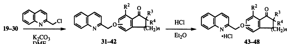
Chart 3. Synthesis of Quinolylmethoxy Ketone Derivatives
