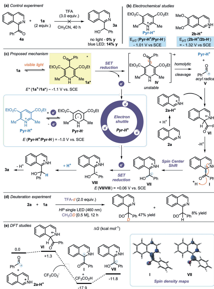
Figure 3. a) Control experiments. b) Redox properties of \text{Pyr-H}^+ (left) and 2\text{b-H}^+ (right). c) Proposed mechanism. d) Deuteration experiment performed in \text{CH}_3\text{OD} using \text{TFA-d} . e) Computed free energy profile for the addition of the benzoyl radical V to isoquinolinium ( 2\text{a-H}^+ ) and subsequent prototropy from VI to VII . Relative free energies are reported in \text{kcal mol}^{-1} at 298 K and 1 atm. Inset: spin density isosurfaces (value = 0.009 e a_0^{-3} ) for I and VII , supporting the SCS process.
