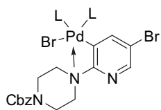
Fig. 2. Chelation of the piperazine nitrogen atom to the Pd species.
