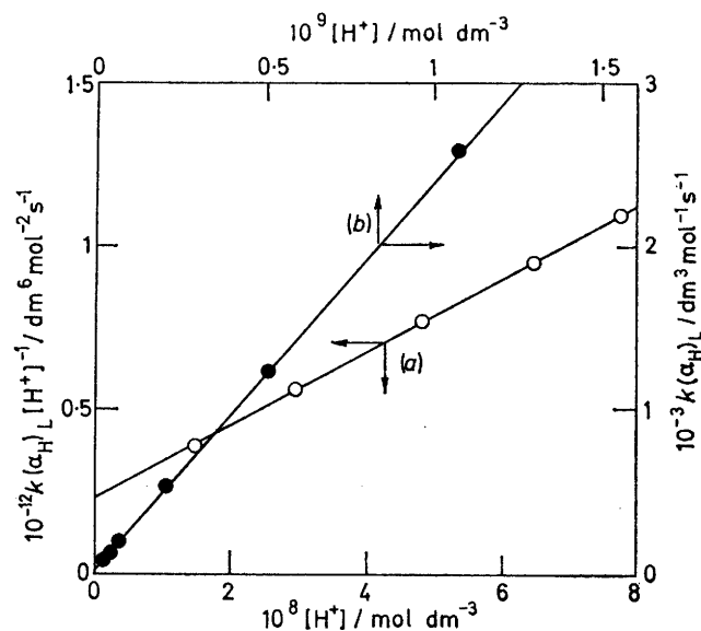
Plots of (a) equation (7) and (b) equation (6) (where K_{\text{CuX}_2}[\text{X}]_F/(\alpha_{\text{H}})_X = 0 for the reaction of [\text{Cu}(\text{edta})]^{2-} with \text{L}^1 )
