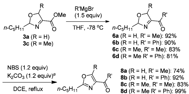
Scheme 5. Preparation of the 4-Keto-oxazole Derivatives
