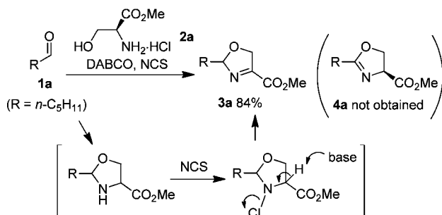
Scheme 3. Formation of the 3-Oxazoline-4-carboxylate 3a
