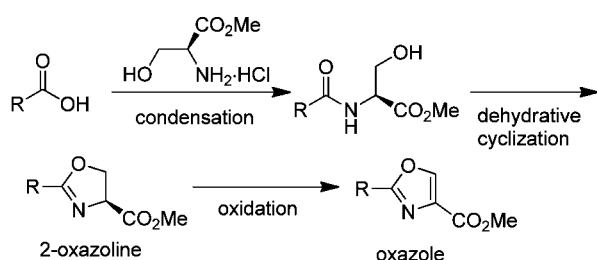
Scheme 1. General Method
