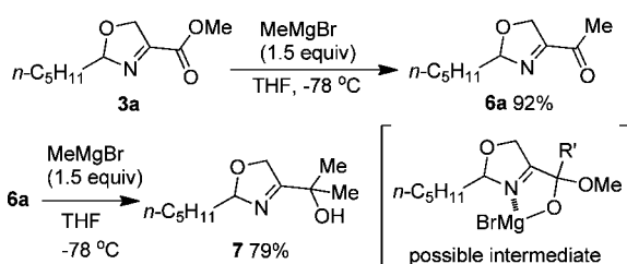
Scheme 4. Reaction of 3a with MeMgBr
