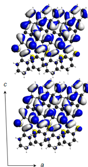
Figure 10. Schematic picture of HOMO distribution in the ac -cell of BTAT: HOMO coefficients are superimposed on the packing structure of BTAT.
