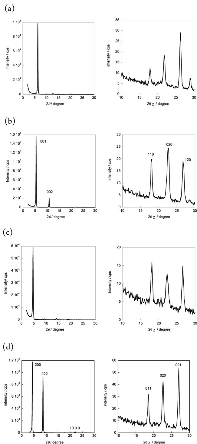
Figure 9. Out-of-plane (left) and in-plan XRD patterns (right) of evaporated thin film on the Si/SiO 2 substrate: (a) BTNT ( T_{\text{sub}} = \text{rt} ), (b) BTAT ( T_{\text{sub}} = 60\text{ }^{\circ}\text{C} ), (c) NTAT ( T_{\text{sub}} = 60\text{ }^{\circ}\text{C} ), and (d) BBTNDT ( T_{\text{sub}} = 100\text{ }^{\circ}\text{C} ).
