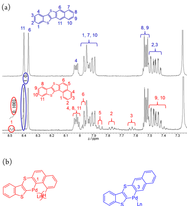
Figure 3. (a) ^1\text{H} NMR spectra of the products (bottom) and authentic BTNT (top), and (b) proposed palladacycle intermediates for both isomers.
