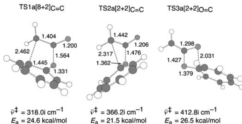
Fig. 1. Three transition states of cycloadditions between tropone ( 1 ) and the parent ketene ( 2a ; R=H). Geometries were optimized with B3LYP/6-31G* calculations. Distances are in Å. \nu^\ddagger is the sole imaginary frequency, which verifies that the obtained geometry is that of the TS.
