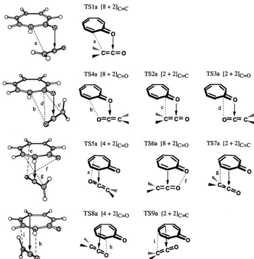
Scheme 6. Nine Cycloaddition Models for Transition-State Searches
