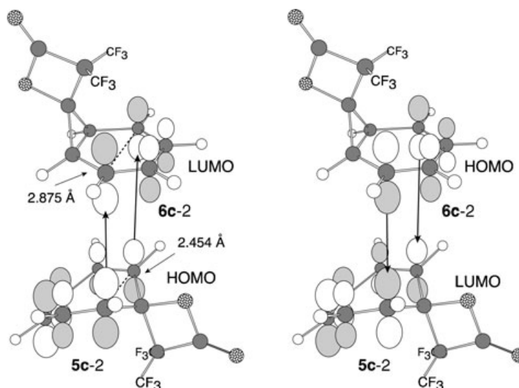
Fig. 9. Antiparallel orientation of 5c-2 and 6c-2 inducing the homo \rightarrow LUMO and HOMO \rightarrow lomo charge-transfer interactions in the [6 + 4] symmetry-allowed orbital overlap. Note that the terminal C \cdots C distances (2.8753 and 2.4535 Å) are similar, which is suitable for the interactions
