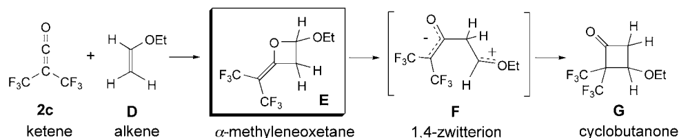
Scheme 4. Reaction between 2c and an Activated Alkene, Ethyl Vinyl Ether D , Involving a Neutral Intermediate E and a Zwitterion F [15]
