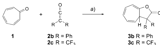
Scheme 7. Reactions of Tropone ( 1 ) with Diphenyl Ketene ( 2b ) or Bis(trifluoromethyl) Ketene ( 2c ) Giving the [8+2] Cycloadducts 3b and 3c
