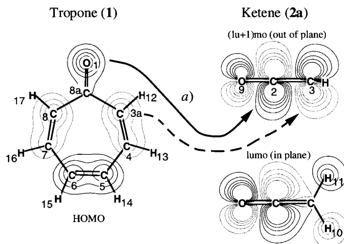
Scheme 5. Frontier-Orbital (Charge-Transfer, CT) Interactions for the Symmetry-Allowed [8+2]_{C=C} Cycloaddition
