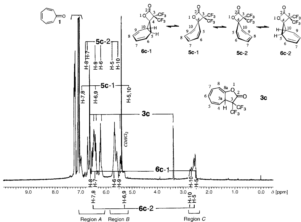
Fig. 5. ^1\text{H} -NMR Spectrum (400 MHz) of [2 + 2] -intermediate \beta -lactones ( 5\text{c-1} \rightleftharpoons 5\text{c-2} \rightleftharpoons 6\text{c-1} \rightleftharpoons 6\text{c-2} ) generated from the reaction between tropone ( 1 ) and bis(trifluoromethyl) ketene ( 2c ). H-5, H-5,10, etc., are short forms of H-C(5), H-C(5) and H-C(10), etc. 4)
