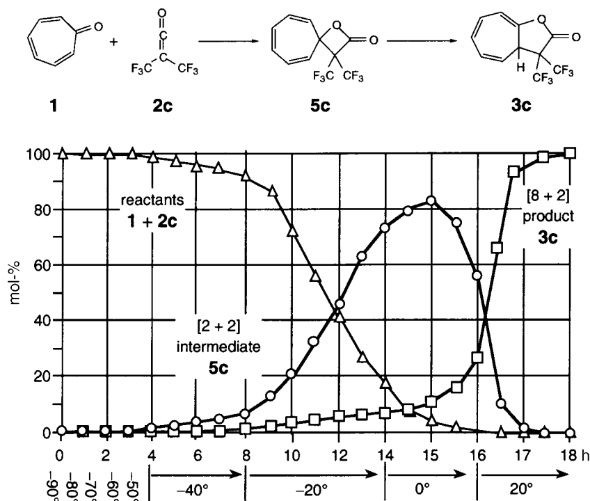
Fig. 2. Variable-temperature 1 H-NMR monitoring of the reaction between tropone ( 1 ) and bis(trifluoromethyl) ketene ( 2c ) in CD 2 Cl 2 . Molar percentages for intermediate 5c take into account the total amount of equilibrium mixture, i.e., cycloheptatrienes 5c-1 and 5c-2 and norcaradienes 6c-1 and 6c-2 (see below)
