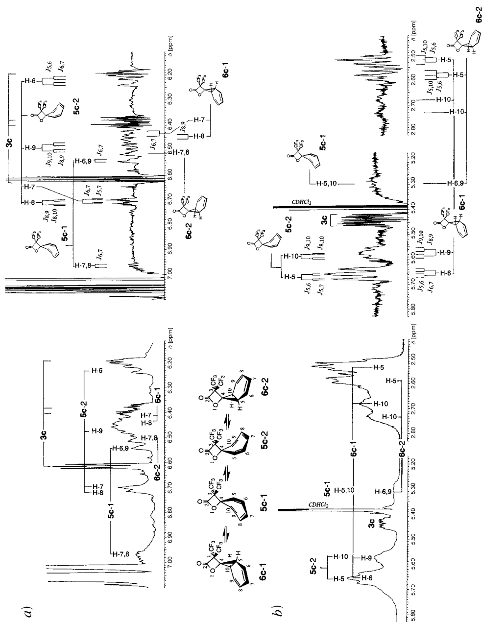
Fig. 6. a) Expansion of Region A ( \delta 7.1–6.1) of the ^1\text{H} -NMR spectrum of Fig. 5 (normal calibration (left) and resolution enhanced with sine-bell wind function (right)). b) Expansion of Region B ( \delta 5.8–5.2) and Region C ( \delta 2.8–2.4) of the ^1\text{H} -NMR spectrum of Fig. 5 (normal calibration (left) and resolution enhanced with sine-bell wind function (right)). H-6, H-6.9, etc., are short forms of H-C(6), H-C(6.9), etc. 4)
