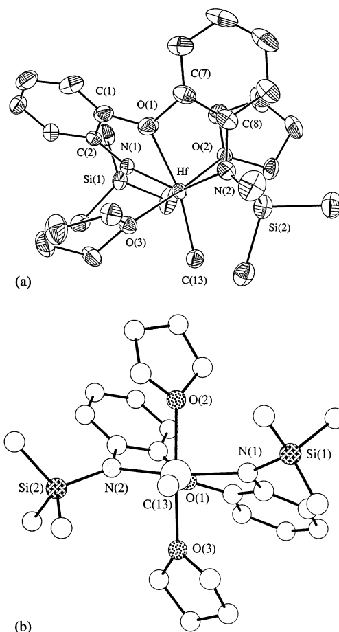
Fig. 1. (a) An ORTEP drawing of the structure of \{[(Me_3SiN- o -C_6H_4)_2O]Hf(CH_3)(THF)_2\}^+ . (b) A CHEM 3D drawing of the structure of \{[(Me_3SiN- o -C_6H_4)_2O]Hf(CH_3)(THF)_2\}^+ .
