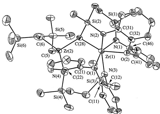
Fig. 2. An ORTEP drawing of the structure of [2][2']\text{Zr}_2(\text{CH}_2\text{SiMe}_3)_2 .
